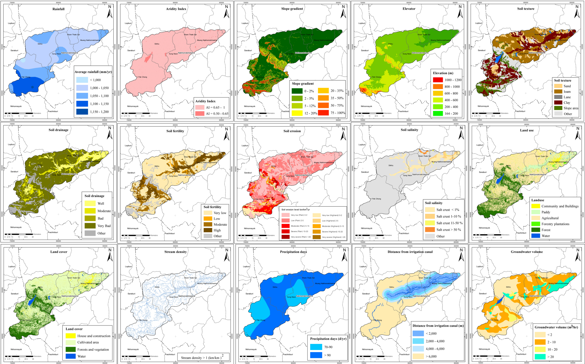
FigureS1. The fifteen risk factors influencing agricultural drought risk in the watershed
