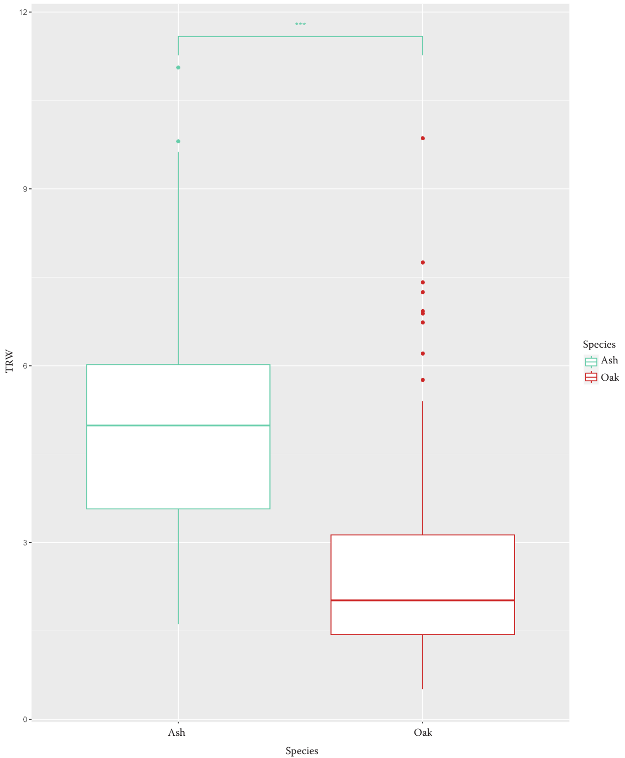
Figure S2. Tree ring width (TRW) since 2015
