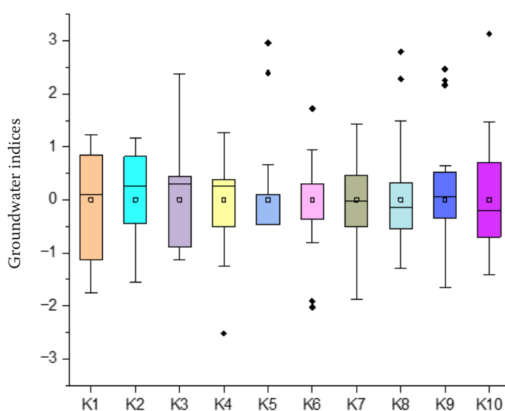
Figure S1. Z-score of underground water level (2019–2022)
