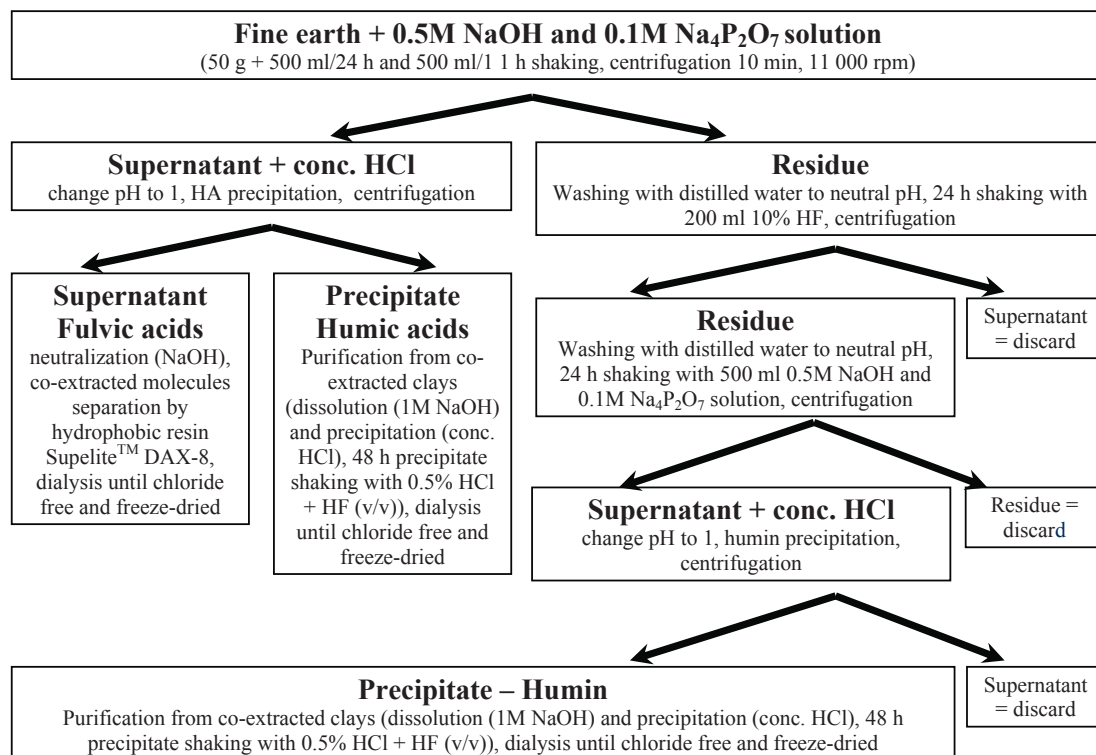
Figure 1. Scheme of humic substances extraction and fractionation
