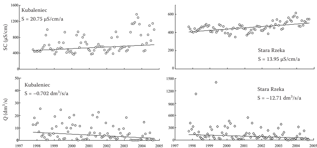
Figure 2. River flow ( Q ) and water specific conductance ( SC ) trend analysis for the Stara Rzeki and Kubaleniec according to Seasonal Kendall Test ( S – Kendall Slope Estimator)
