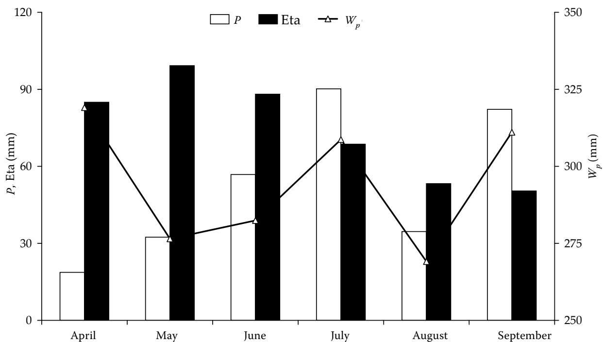
Figure 4. Monthly precipitation totals ( P ) actual evapotranspiration ( E_t ) and the regime of the mean monthly values of soil water storage ( W_p ) in individual months of 2003 vegetation period under the maize growth at the locality Milhostov; GWL = 110–150 cm; WP – wilting point
