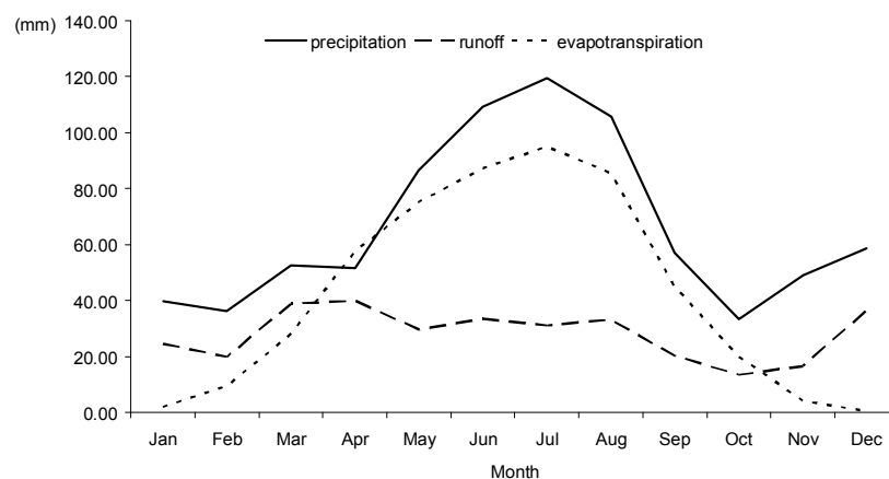
Figure 13. Runoff, precipitation, and evapotranspiration in the subbasin (No. 29), where the hydrotop of the highest evapotranspiration is located
