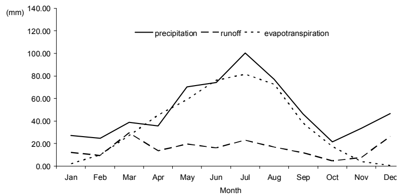
Figure 14. Runoff, precipitation and evapotranspiration in the subbasin (No. 7), where the hydrotop of the lowest evapotranspiration is located
