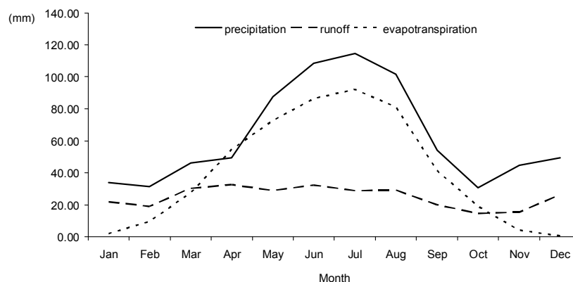
Figure 15. Runoff, precipitation and evapotranspiration in the subbasin (No. 28), where the hydrotop of the average evapotranspiration is located
