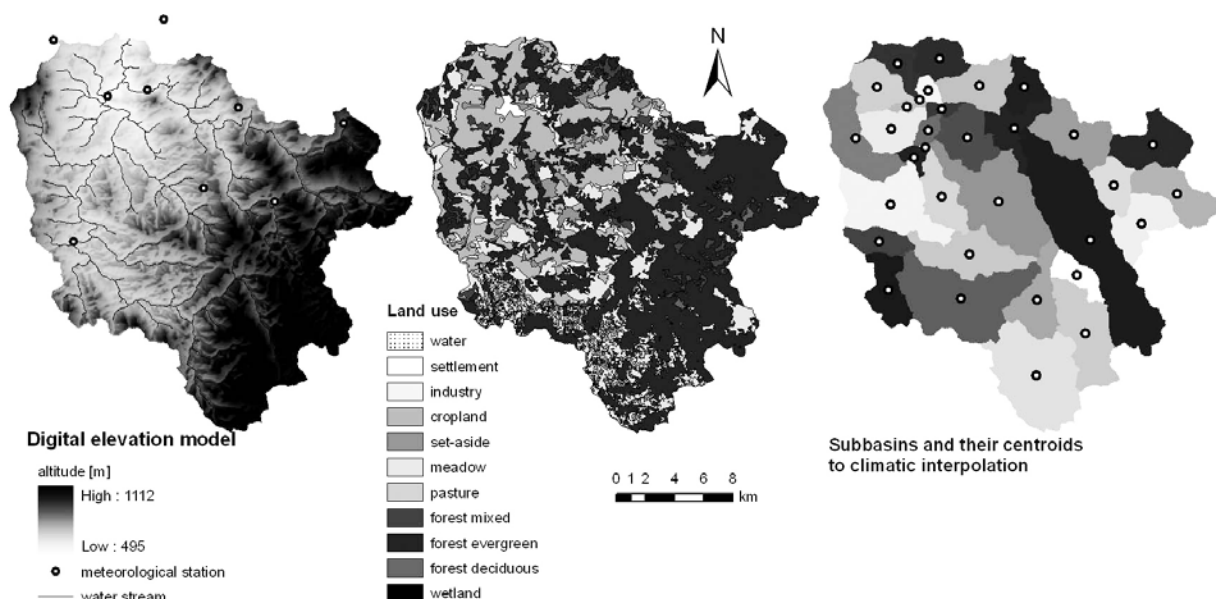
Figure 2. The Malše River basin input maps (elevation, land use, subbasins with their centroids)
