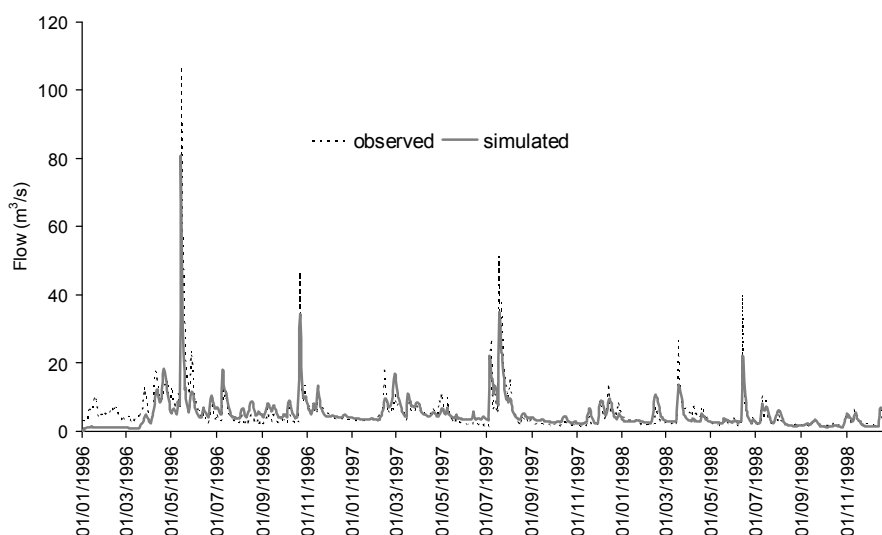
Figure 4. Observed and simulated flows during validation period
