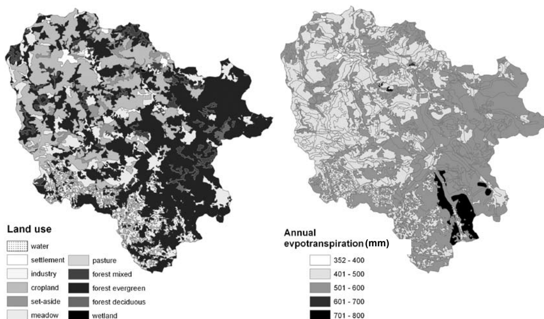
Figure 5. Comparison of the map of the average annual evapotranspiration (mm) with the map of land use
