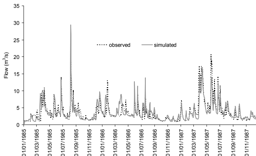
Figure 3. Observed and simulated flows during calibration period
