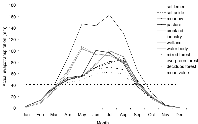
Figure 11. Annual course of actual evapotranspiration in different land use types
