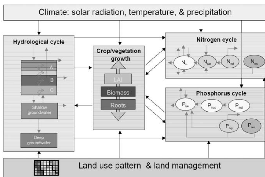
Figure 1. Flow chart of the SWIM model (KRYŠANOVÁ et al. 1998)
