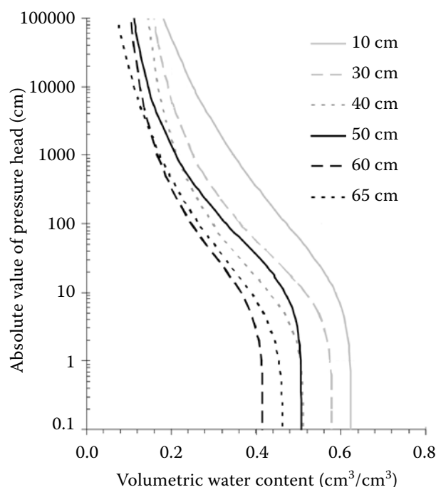
Figure 2. Reference retention curves determined for 6 depths
