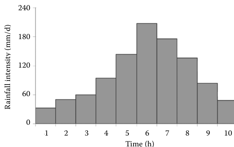
Figure 1. 10-hour synthetic rainfall event; during the first 10 h of simulation period, the synthetic extreme rainfall event is applied as a top boundary condition
