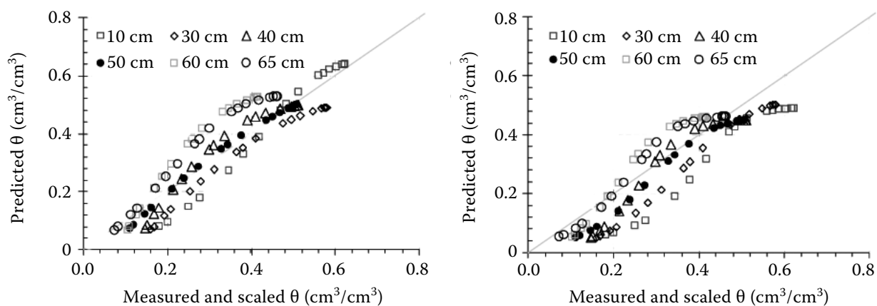
Figure 3. Comparison of the measured reference retention curves and the retention curves predicted by PTFs; graph on the left: measured vs. retention curve predicted by PTF of WÖSTEN et al. (1999); graph on the right: measured vs. retention curve predicted by PTF of SCHAAP et al. (1998)
