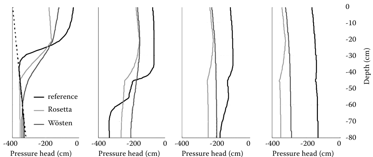
Figure 4. Simulated pressure head profiles for times 6, 12, 24, and 72 hours; initial distribution of pressure (dashed line) is shown in the graph on the left
