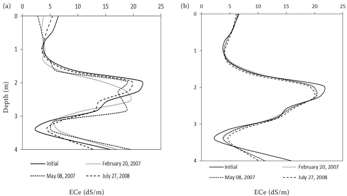
Figure 4. Effect of exceptional rain (50 mm/day) on salts dynamics; (a) with 50 mm/day, (b) without 50 mm/day
