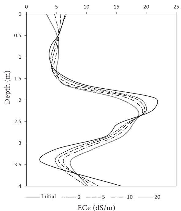
Figure 5. Long-term simulation of saline profile
