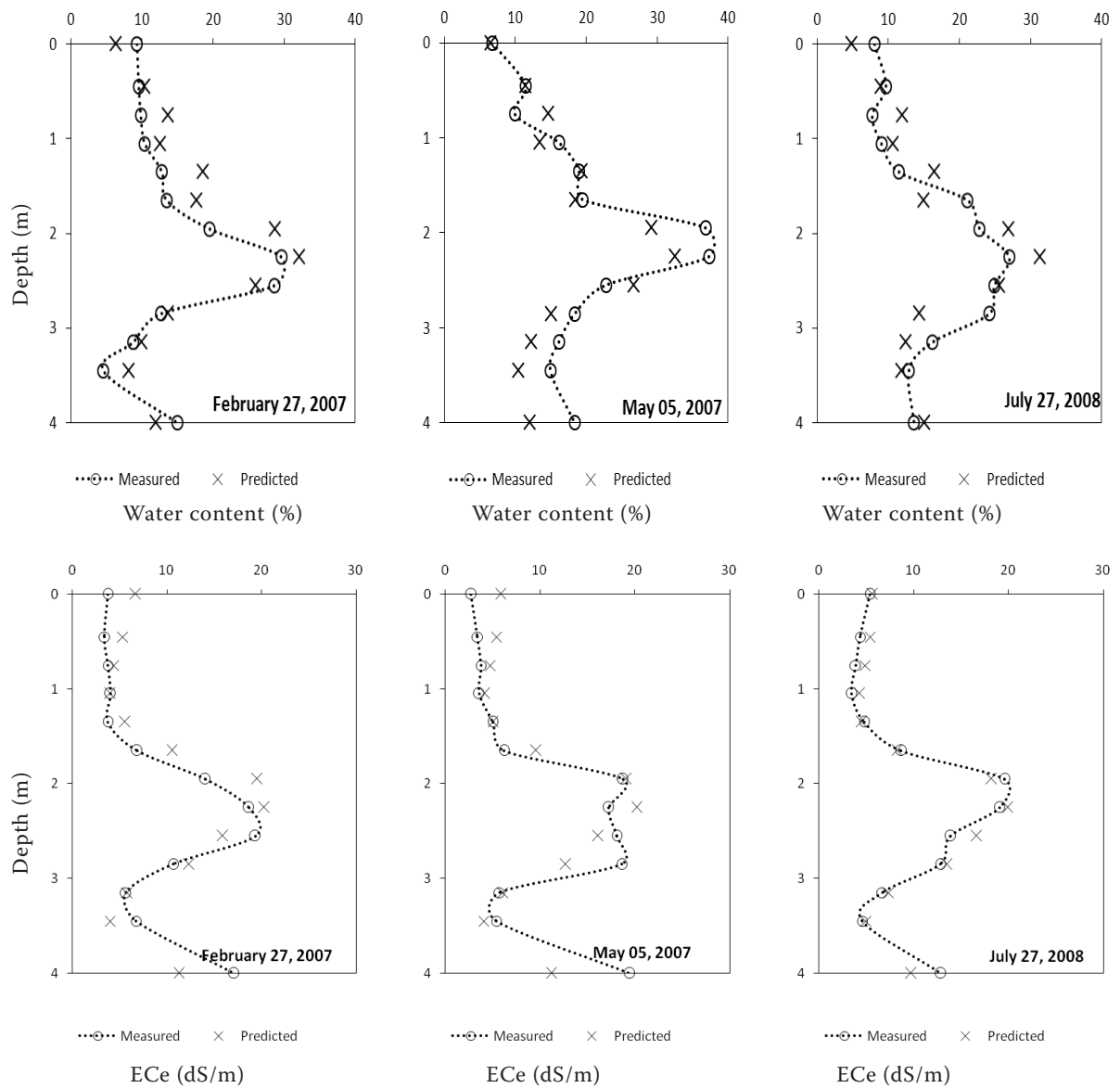
Figure 3. Measured and predicted profiles for each output time
