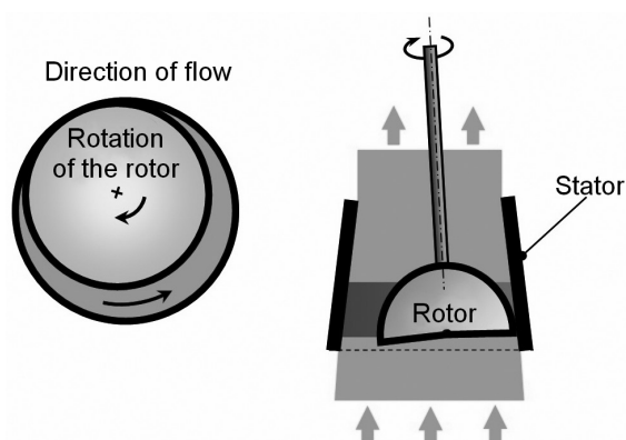
Figure 1. Principle of bladeless turbine (POLÁK et al. 2013)
