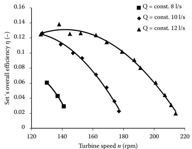
Figure 6. Dependence of output power on turbine speed at different flow rates
