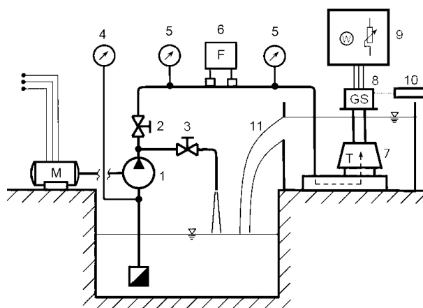
Figure 3. Diagram of the hydraulic circuit for measuring the DVE 120 miniturbine (DLABAL et al. 2015)
