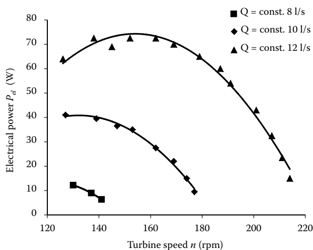
Figure 5. Dependence of usable water gradient on turbine speed
