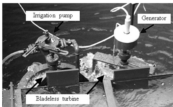
Figure 2. Bladeless turbine in conjunction with an irrigation pump and an electric generator (HOSTIN et al. 2005)
