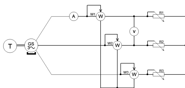
Figure 4. Electrical circuit wiring
